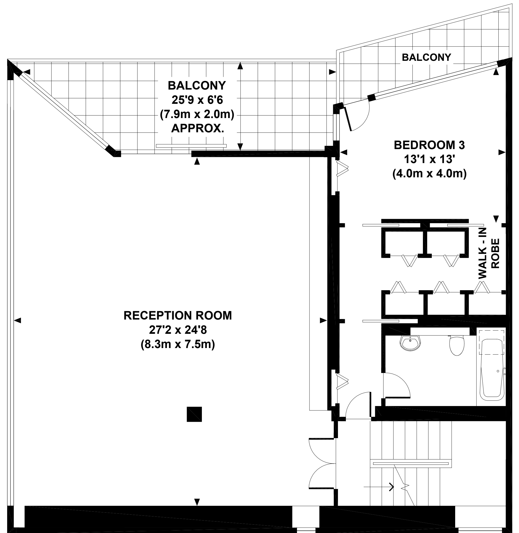
FIRST FLOOR
